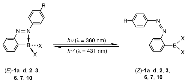
Scheme 4. Irradiation of 2-(phenylazo)phenylboranes ( E )- 1a–d , 2 , 3 , 6 , 7 , and 10 in \text{C}_6\text{D}_6 .
