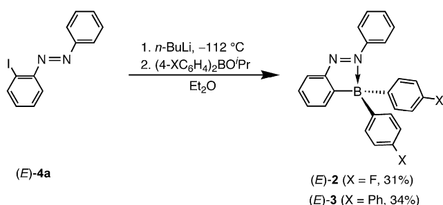
Scheme 2. Synthesis of ( E )- 2 and ( E )- 3 .
