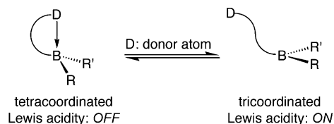
Scheme 1. Switching of the coordination numbers of the boron and the Lewis acidity by using an intramolecular bidentate and bistable ligand.
