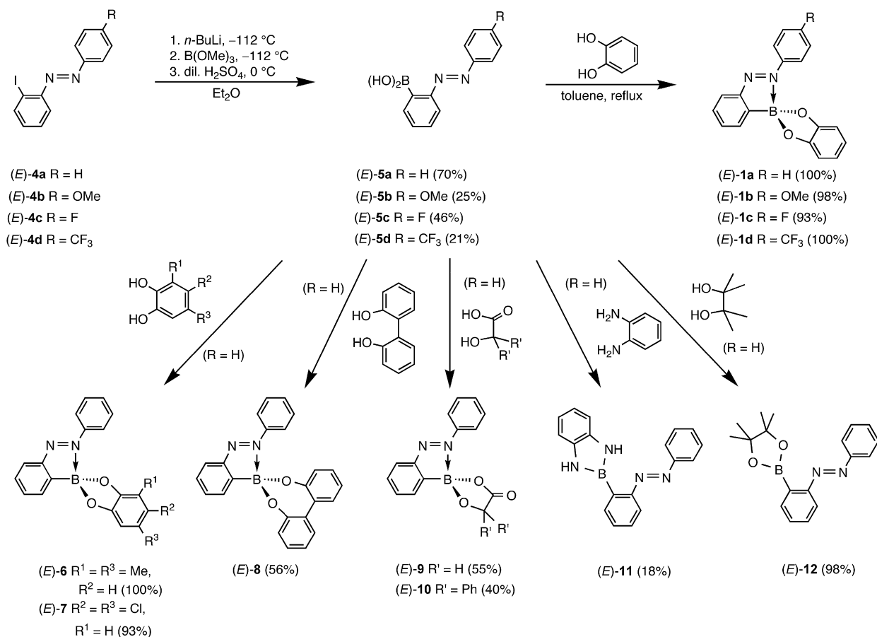
Scheme 3. Synthesis of ( E )- 1a–d , 5a–d , and 6–12 .
