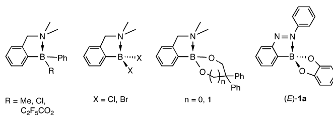
Figure 1. Tetracoordinated boranes with 2-(dimethylaminomethyl)phenyl group and 2-(phenylazo)phenyl group.
