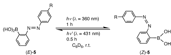
Scheme 5. Irradiation of boronic acid ( E )- 5a–d in \text{C}_6\text{D}_6 .
