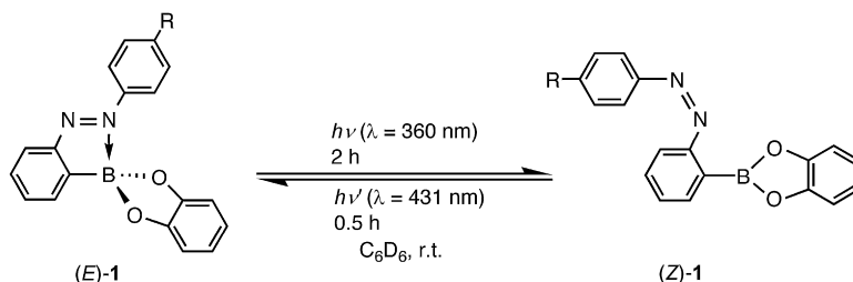
Scheme 6. Irradiation of catecholborane ( E )- 1a–d in C_6D_6 .
