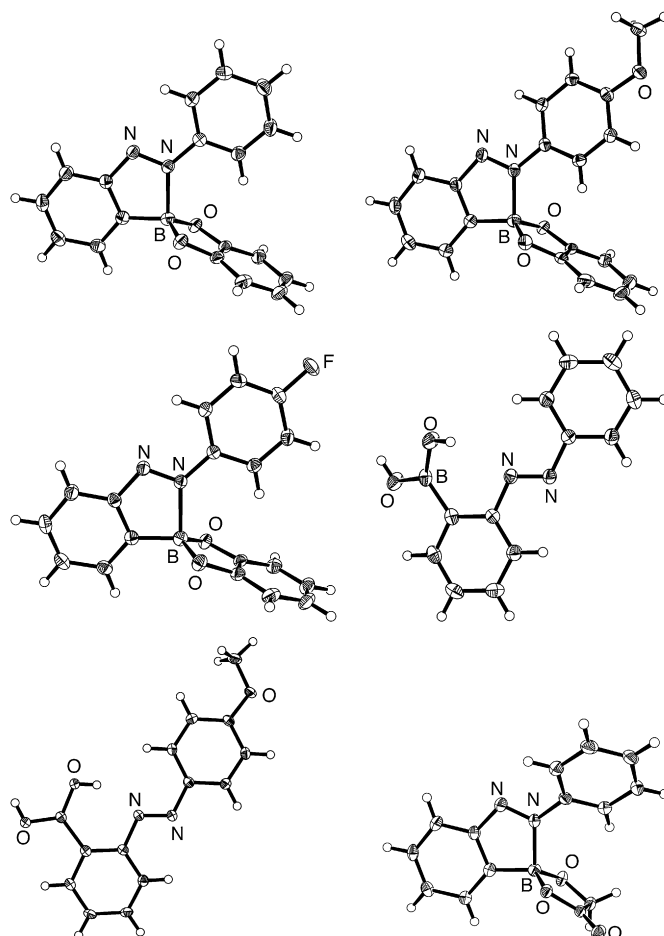
Figure 2. ORTEP drawings of ( E )- 1a (top-left), 1b (top-right), 1c (middle-left), 5a (middle-right), 5b (bottom-left), and 9 (bottom-right).
